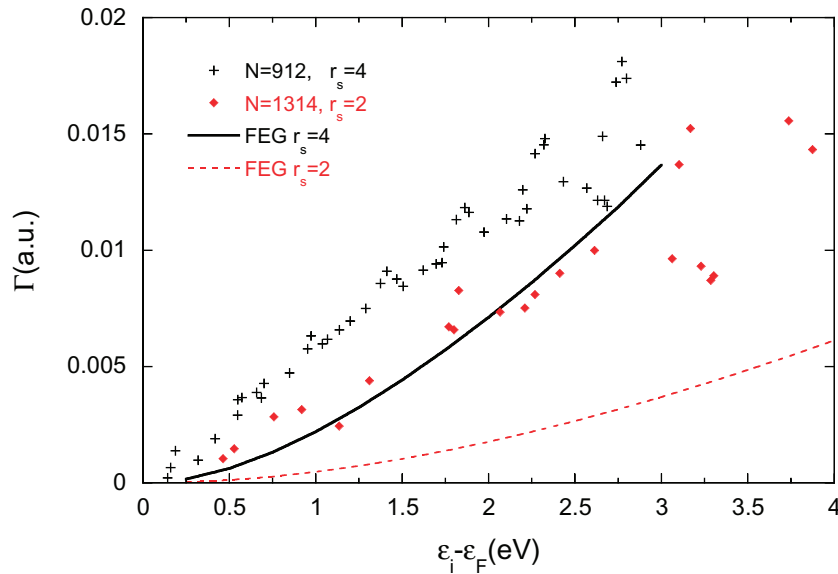
Figure 2. Decay rate \Gamma = \tau^{-1} for electronic excitations in nanoparticles as a function of the excitation energy \varepsilon_i - \varepsilon_F . (Red) diamonds refer to a nanoparticle of N = 1314 and r_s = 2 ( R = 1.1 nm). (Black) crosses refer to a nanoparticle of N = 912 and r_s = 4 ( R = 1.9 nm). The dashed (red) line and the solid (black) line show the values of \Gamma in an infinite electron gas of r_s = 2 and r_s = 4 , respectively.
