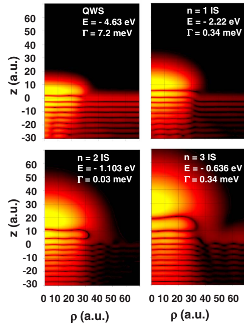
FIG. 2. (Color online) Interpolated images of the electron density of the (m=0, j=0) quasistationary island-localized states for the 61 Na atom island on the Cu(111) surface. The states are labeled according to their parent continua. The natural logarithm of the density is shown in cylindrical coordinates. z=0 corresponds to the position of the image plane of the Cu(111) surface, and inside the metal z is negative. The vacuum edge of the Na island is at z=5.0 a.u. The electron density decreases from 1 to 0.001 (arbitrary units) when going from bright to dark. The energies E [with respect to the vacuum level of Cu(111)] and the widths \Gamma of the states are given in the insets.
