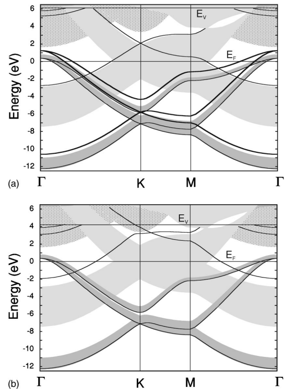
FIG. 1. Projected bulk band structure of MgB 2 together with the surface and image-potential states for B-terminated (a) and Mg-terminated (b) surfaces. The light (dark) grey areas represent the \pi ( \sigma ) projected bulk states. Dotted areas indicate the magnesium projected states. Thick solid lines depict surface states which are mostly localized in the topmost B layer.
